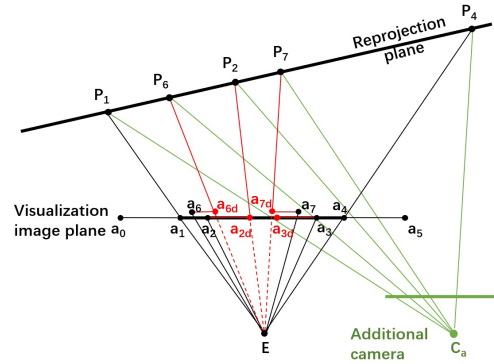
Figure 5. The sampling of the general pinhole camera model for zooming in for AR scenes
