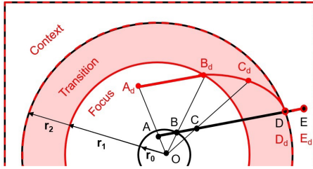
Figure 3. The projection displacement of the FPC model.
